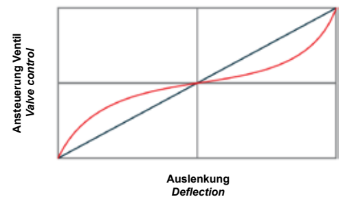
Kennlinie / Characteristic
